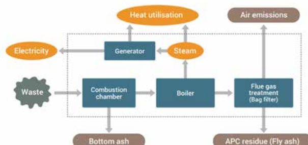
Figure 1: Typical flow chart of WtE incineration plant © IGES
